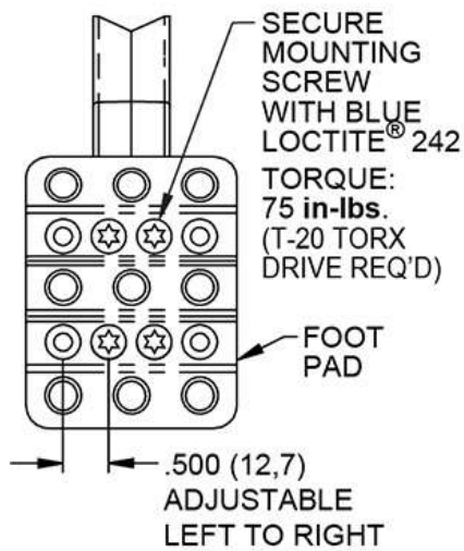
FOOT PAD DETAIL
